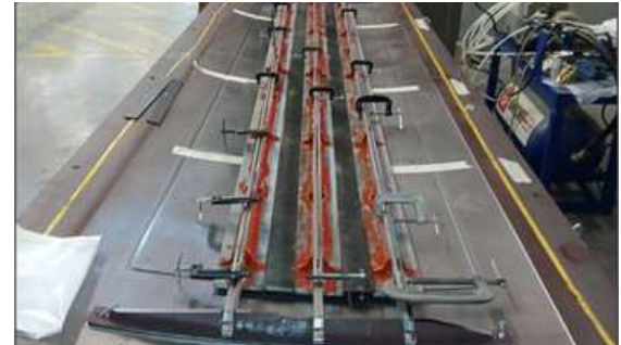
Mold tool for upper stiffed panel: Final fit check by LDO and HAI
