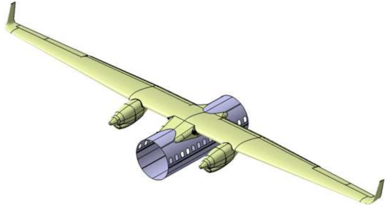
Digital mock up of the UERA wing with the integration of the nacelle shared by HERA project for the D2-4 (Full wing virtual test) simulation
