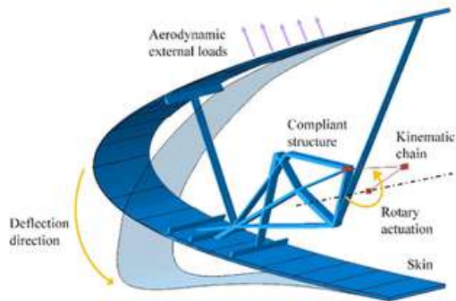
Morphing Droop Nose functionality concept
