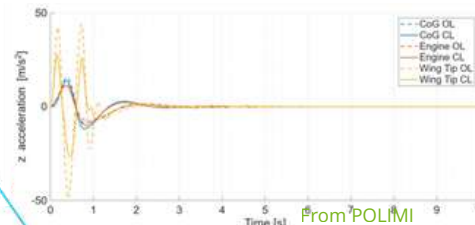
Figure 13: Accelerations at different locations
