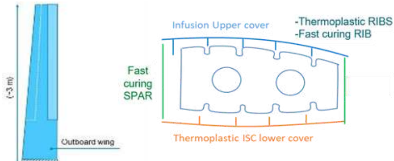
Outer wing box demonstrator
