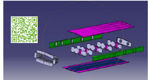
HERWINGT Demo series, Outer Wing Box Demonstrator (E02)
