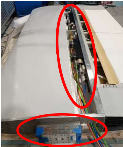
RUAG balance and motor measurements
