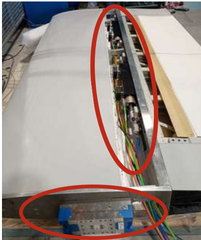
RUAG balance and motor measurements
